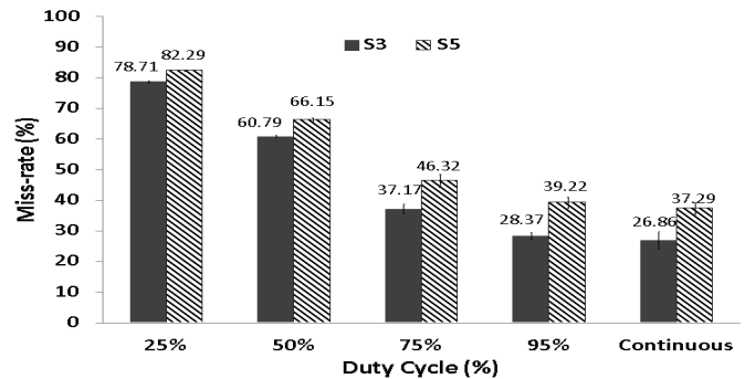
Fig. 3. BLE Miss Rates (BLE-Active Environment), ( T_s = 1\text{sec} )
